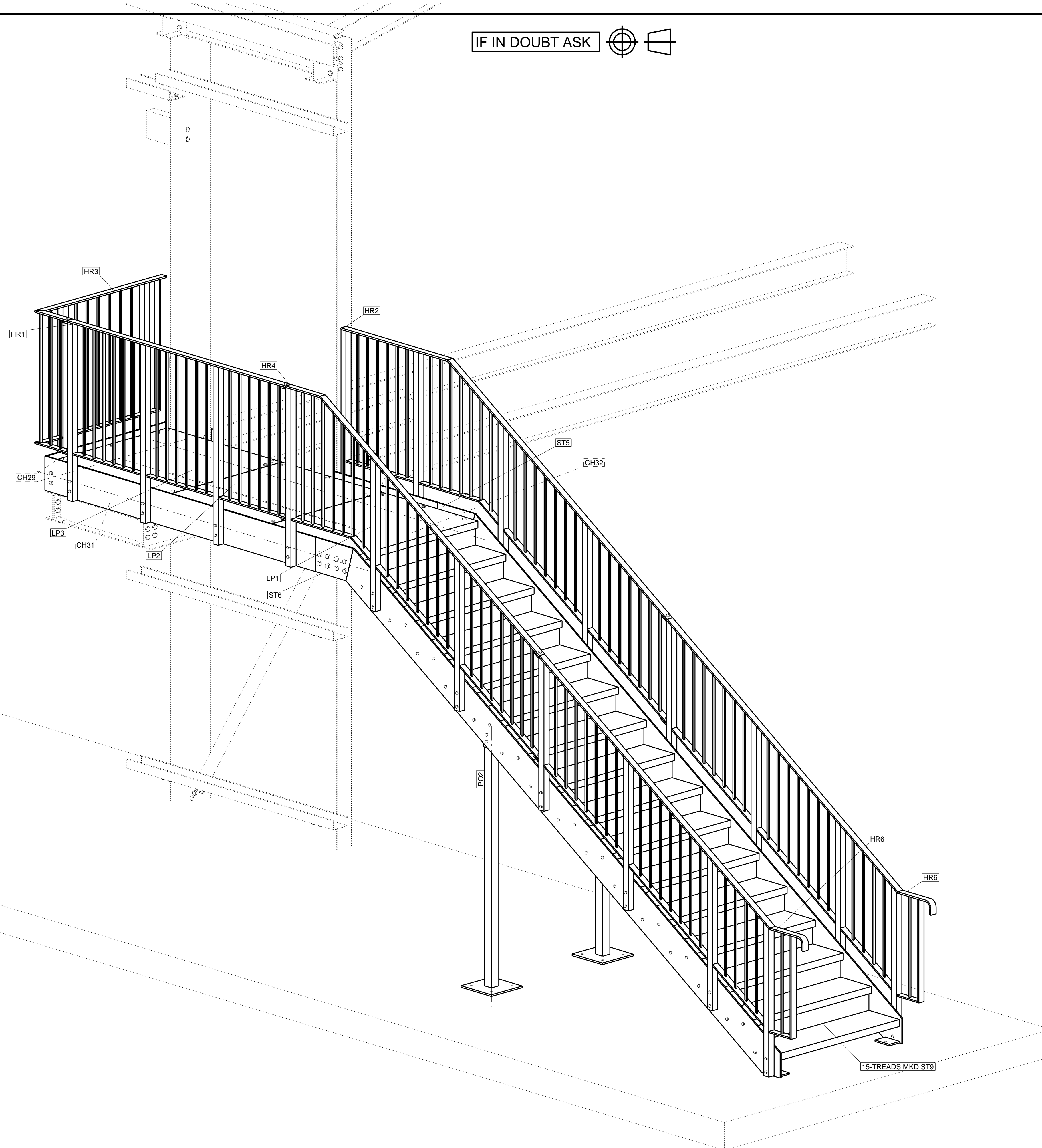
3d View Of South Workshop Stairs
