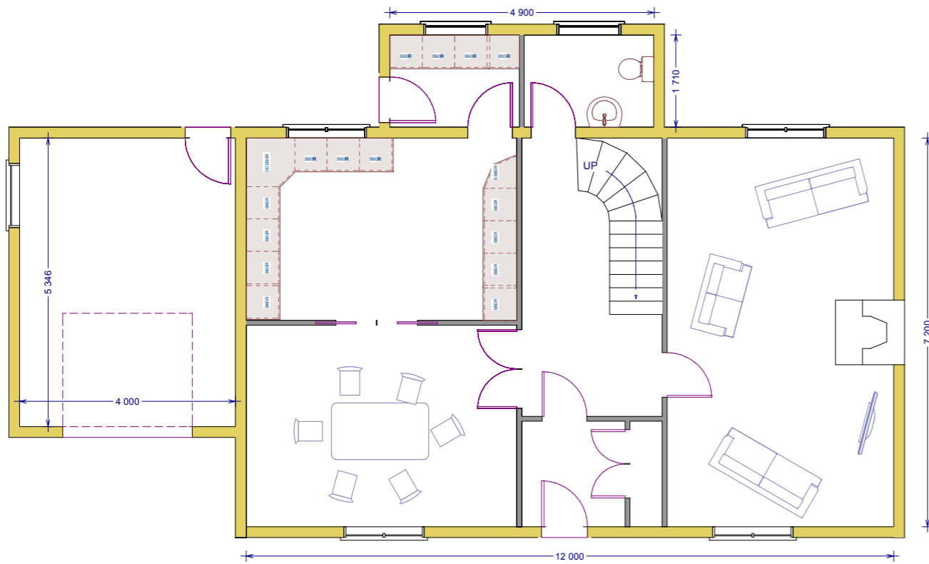
Ground Floor
